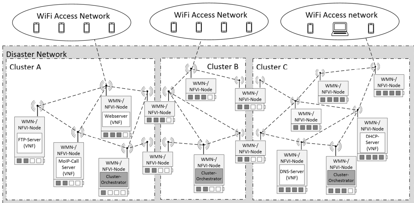
Figure 2 – Normal State of the WMN-based Disaster Network
